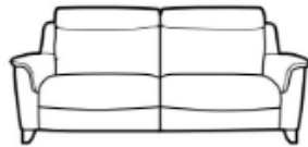
LARGE TWO SEATER (HEATED SEATS AVAILABLE) H 102cm W 199cm D 104cm SH 49cm SW 153cm SD 49cm AH 64cm
