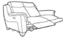
LARGE TWO SEATER POWER RECLINER (HEATED SEATS AVAILABLE)(POWER OR POWER PLUS AVAILABLE) H 102cm W 199cm D 104cm SH 49cm SW 153cm SD 49cm AH 64cm FULL RECLINE 164cm
