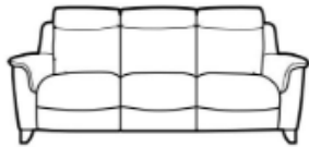
THREE SEATER (HEATED SEATS AVAILABLE) H 102cm W 222cm D 104cm SH 49cm SW 176cm SD 49cm AH 64cm
