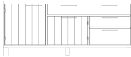
LARGE SIDEBOARD H 800 W: 1520 D: 430
