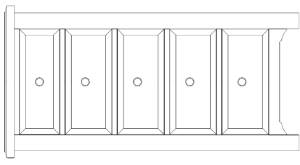
5 DRAWER WELLINGTON CHEST H: 1,218 W: 630 D: 430
